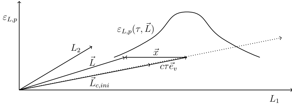
Figure 6.5: Sketch of a localizable portion of relative additional volume \varepsilon_{L,p} . The center is at \vec{L}_c = \vec{L}_{c,ini} + c \cdot \tau \cdot \vec{e}_v . A location is represented by \vec{x} relative to the center and by \vec{L} = \vec{L}_c + \vec{x} relative to the origin. In empty space, according to translation invariance, the DEQ of VD also holds for each such off-center \vec{L} .
