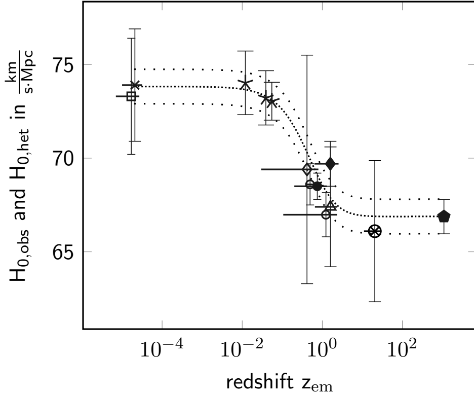
Figure 16.4: Observed values H_{0,obs} and derived values H_{0,het} of H_0 as a function of z_{em} .
