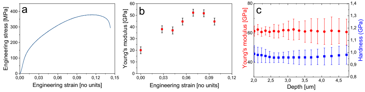
Fig. 2. Young's modulus extracted from the load-unloading stress-strain curve probed under compression and plotted as function of strain; (c) Young's modulus and hardness probed by nanoindentation.
