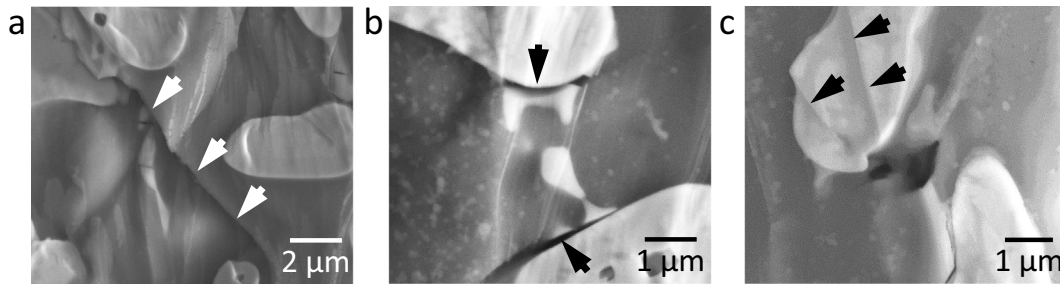
Fig. 4. Ex-situ SEM micrographs of the Fe-Mg composite after strain of 0.1. (a) Slip bands passing through the Mg phase, marked by arrows; (b) Detachment of the Mg 2 Ni and Fe as well as Mg and Fe phases, marked by arrows; (c) Slip bands passing through the Fe phase, marked by arrows.
