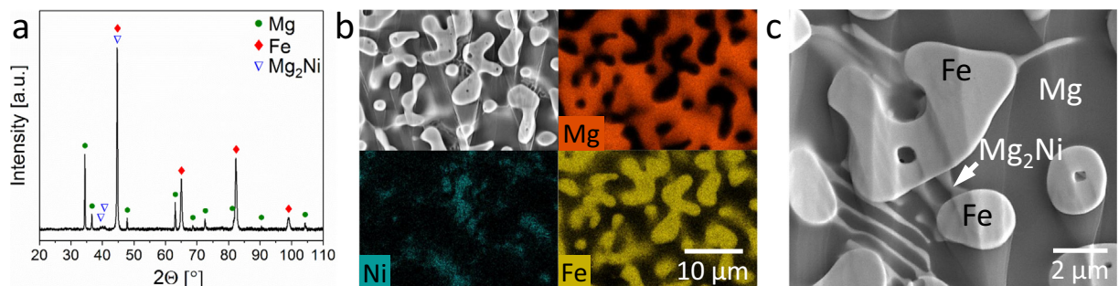
Fig. 1. X-Ray diffraction pattern (a) and secondary electron micrographs together with elemental mapping (b and c) of the Fe-Mg composite fabricated from Fe_{30}Ni_{70} precursor alloy (at. %) by dealloying in liquid Mg at 1023 K for 30 min.
