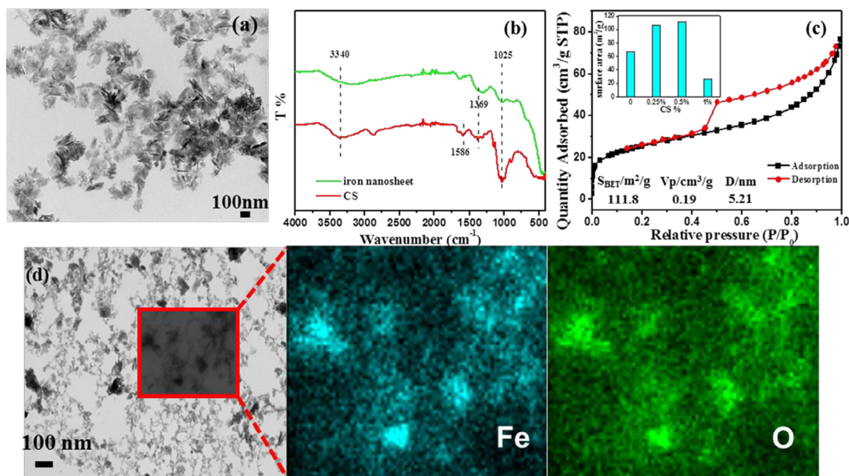
Fig. 1. TEM images (a), FTIR spectrum (b), N 2 adsorption/desorption isotherms with surface area and pore size information (c) and the corresponding element mapping images of Fe and O in the rectangular region (d) for the as-prepared iron nanocomposite with 0.5 wt% CS. And the inset in figure c shows the surface areas of samples as a function of CS content.
