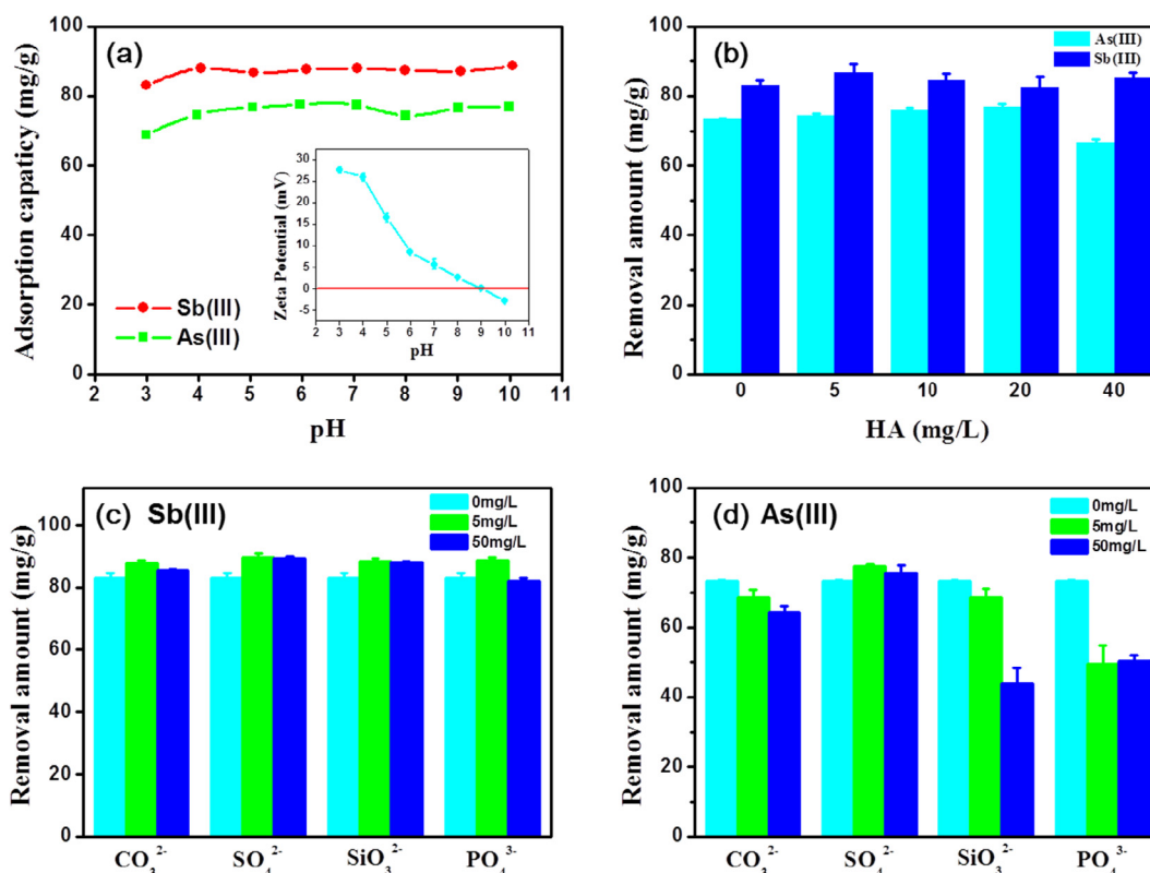
Fig. 4. (a) As(III) and Sb(III) removal by the iron nanocomposite as a function of pH values and the inset in a is the zeta potential. Effect of HA (b) and anions (c and d) on the removal of As(III) and Sb(III), including CO 3 2- , SO 4 2- , SiO 3 2- and PO 4 3- (initial concentration of As(III) and Sb(III): 40 mg/L; adsorbent dosage: 0.4 g/L; pH: 7).
