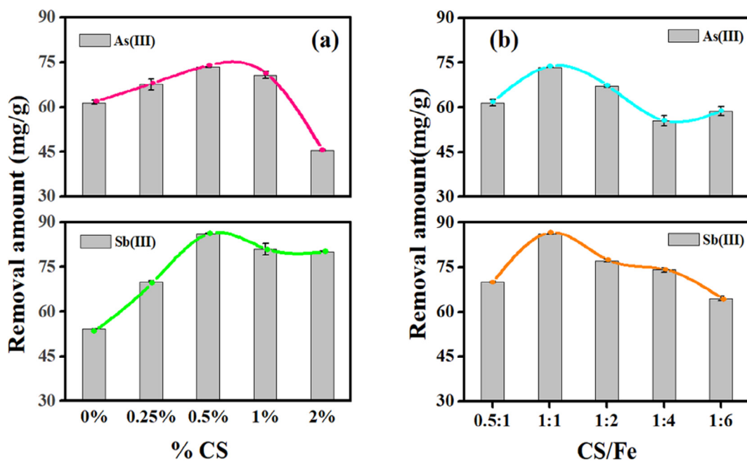
Fig. 2. (a) Effect of varying CS content; (b) effect of the CS/Fe ratio on the adsorption of As(III) and Sb(III).
