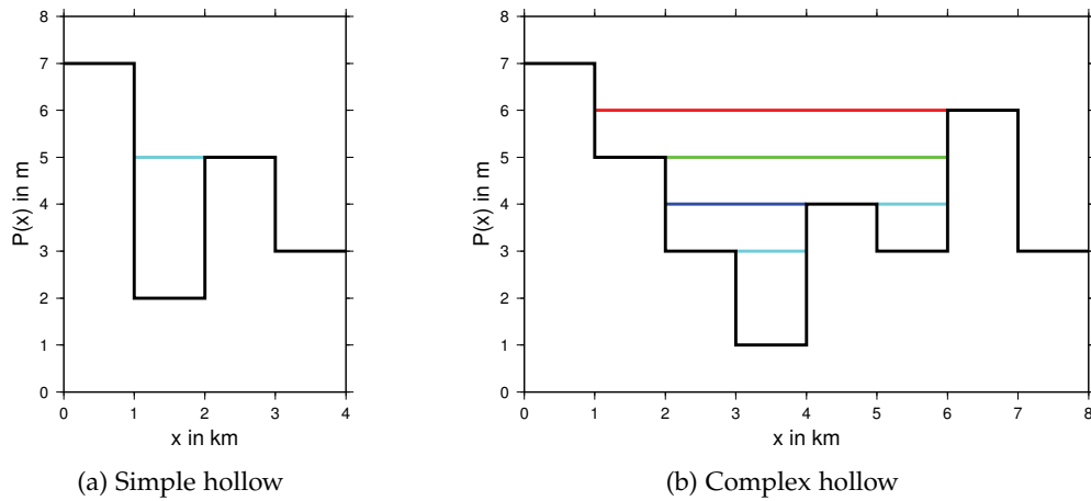
Figure 15: Hollow filling algorithm, applied to a one-dimensional hydraulic potential P(x) : (a) Simple hollows are set to their lowest neighbor (cyan). (b) More complex hollows are iteratively filled up (in the following order: cyan, blue, green, red). The concept can be extended for the application to two-dimensional hydraulic potentials.
