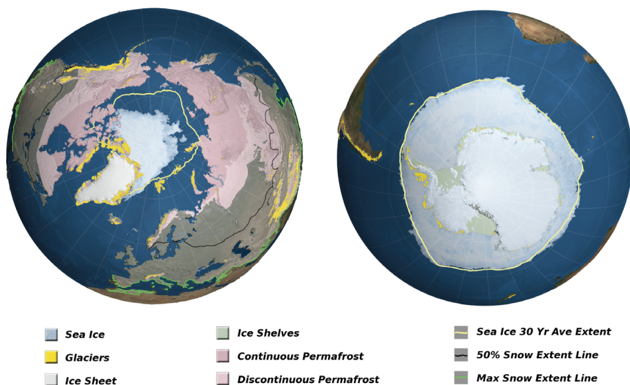
Figure 1: Components of the Earth’s cryosphere in the Northern and Southern Hemisphere (Fig. after Goddard Space Flight Center, 2011 ).
