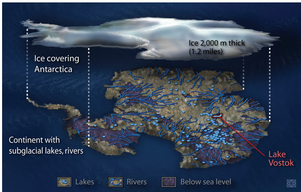
Figure 3: Beneath the AIS 379 subglacial lakes have been discovered so far. They are connected by subglacial rivers and form a widespread hydrological network which influences the dynamics of the overlaying ice. The largest subglacial lake is Lake Vostok. (Fig. by National Science Foundation, 2007b)
