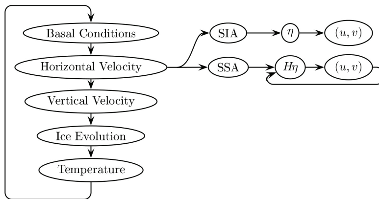
Figure 7: Sequence of iteratively solved variables for SIA and SSA (here the product H\eta is calculated, instead of \eta ) within RIMBAY (Fig. after Thoma et al., 2014 ).
