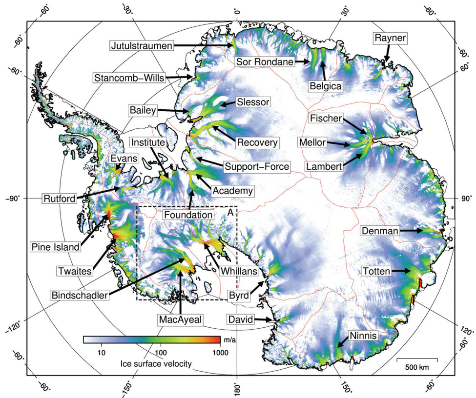
(a) Ice surface velocities for grounded ice (Rignot et al., 2011a)
