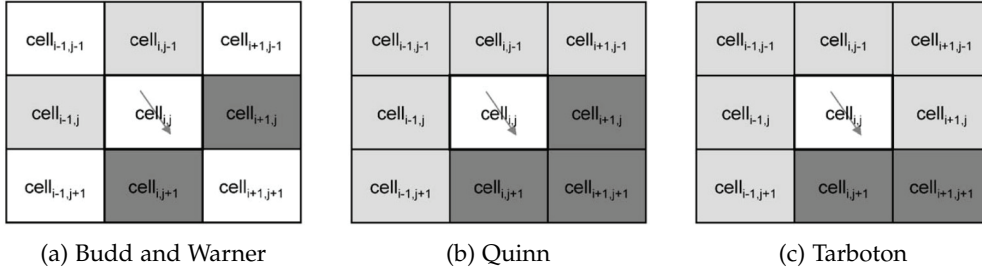
Figure 16: Schematic diagrams to illustrate the differences of the algorithms by (a) Budd and Warner (1996) , (b) Quinn et al. (1991) and (c) Tarboton (1997) . For the central grid cell (i, j) the flow direction \theta_{i,j} is indicated by an arrow, the potentially water-contributing grid cells are marked in light gray and the water receiving grid cells in dark gray (Figures by Le Brocq et al., 2006 ).
