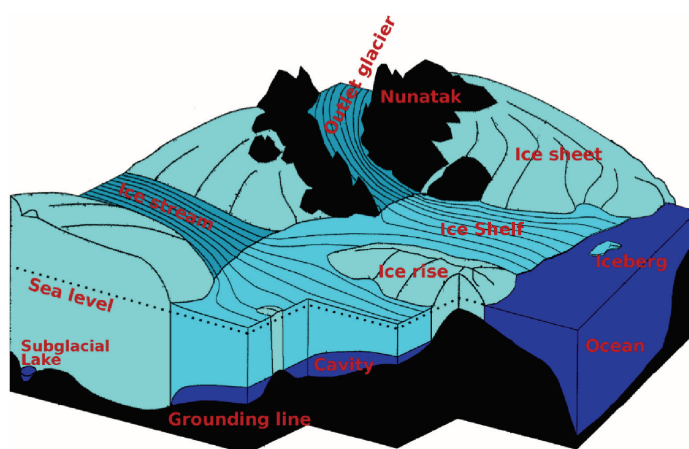
Figure 5: Schematic illustration of several features which belong to an ice sheet/shelf system, e.g., the Antarctica Ice Sheet with its shelves, and have to be considered in modeling approaches (Fig. after Sandhäger, 2000 ).
