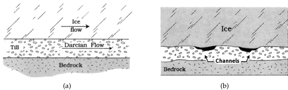
Figure 14: Distributed water flow: (a) Darcian flow within till or sediment at the ice base. (b) Flow in wide, shallow and ice-roofed channels cut into the till. (Figures after Fountain and Walder, 1998)
