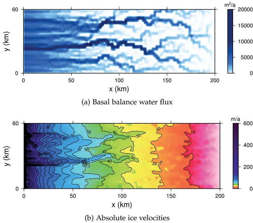
Figure 42: Balanced water layer concept with lake- and flux-sliding coupling (BWF)
