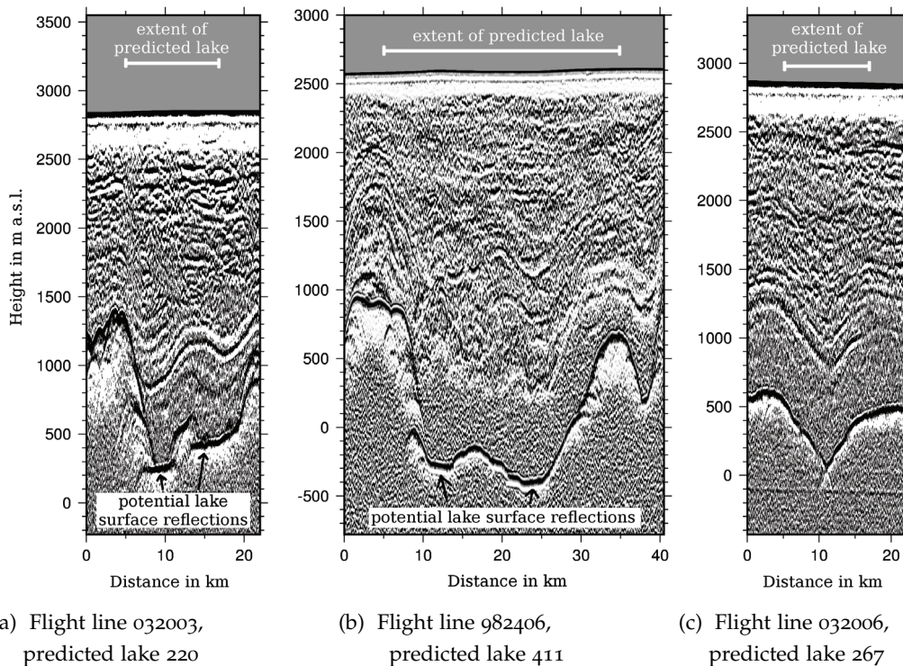
Figure 24: Selected radar profiles of AWI RES flight lines crossing predicted and so far uncharted subglacial lakes (Fig. 23). All three profiles show a hollow in the bedrock topography in good agreement with the predicted maximum possible lake extent. Profile (a) and (b) show strong and flat lake-like radar reflections at the bottom of the bedrock troughs. The basal reflections in profile (c) show no indications for the existence of accumulated basal water.
