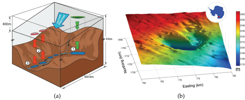
Figure 11: Active subglacial lakes: (a) Schematic illustration of correlated ice surface lowering (green) and uplift patterns (red) above adjacent subglacial lakes indicating that these lakes are linked (Fig. by SCAR). (b) Ice sheet surface deformation caused by the drainage of subglacial Lake Cook, mapped by CryoSat-2 interferometric mode data (Fig. after McMillan et al., 2013).
