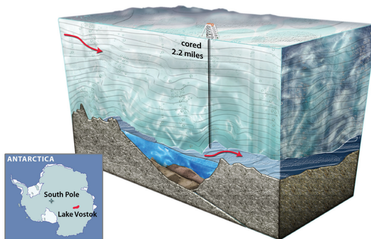
Figure 8: Schematic cross section of Lake Vostok beneath the East Antarctic Ice Sheet, the largest known subglacial lake (Fig. by National Science Foundation, 2007a ).
