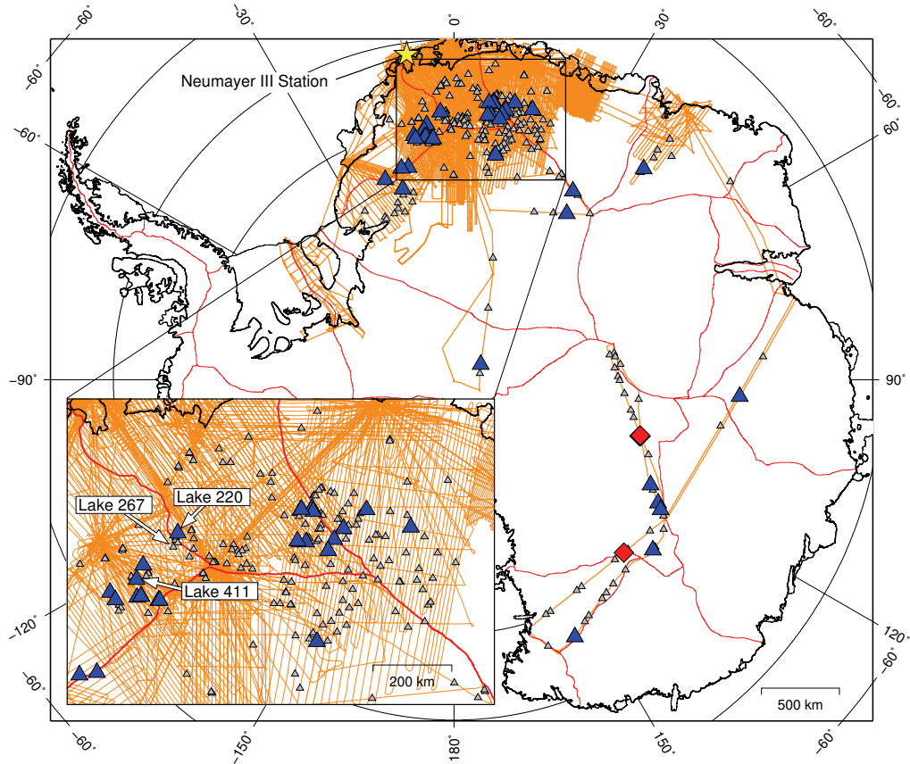
Figure 23: All AWI RES flight lines (orange) in Antarctica from 1994 to 2013 with locations marked by triangles where flight lines cross the outline of a predicted subglacial lake. Red diamonds indicate predicted and already known subglacial lakes (Lake Vostok and Adventure Trench Lake) ascertained by a clearly visible lake surface reflection in the associated radar profile. Gray triangles stand for predicted and so far uncharted subglacial lakes where no lake-surface could be detected in the radar profiles. Predicted and so far uncharted subglacial lakes where a potential lake surface reflection is found in the radar profile are pointed out by blue triangles. For three selected predicted lakes the radar profile is shown in Fig. 24. Coast and grounding line (black) by NSIDC and ice divides (red) by AGAP.
