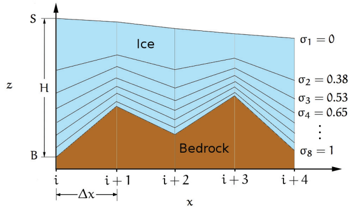
Figure 6: Schematic cross-section of an ice sheet as an example: terrain-following \sigma -coordinates which become closer from the ice surface elevation S towards the bedrock elevation B . The ice thickness is given by H = S - B .
