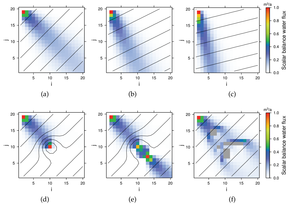
Figure 17: Scalar balance water flux on an inclined plane following the Budd and Warner (1996) scheme (Fig. 16a) by RIMBAY. Only at grid cell (i, j) = (2, 19) a basal melt rate M_b of 1 \text{ m a}^{-1} is defined. The hydraulic potential is illustrated by its equipotential lines. (a-c) Flux for different grid orientations. (d) Flux is ending in a hollow of the hydraulic potential. (e) Flux crosses the hollow after modification of the hydraulic potential. (f) Flux is directed around obstacles, e.g., Nunataks (gray).
