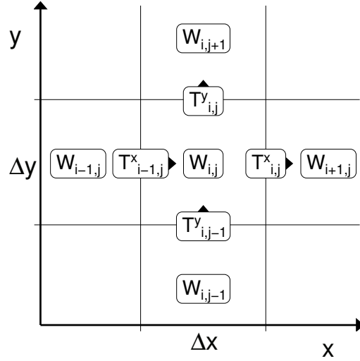
Figure 37: Notation for staggered Arakawa C-grid: at the grid center: basal water layer thickness W_{i,j} , hydraulic potential P_{i,j} , normalization N_{i,j} , water flux \phi_{i,j} (for coupling to an A-grid ice model), at the grid cell edges: water transport T_{i,j}^x and T_{i,j}^y , hydraulic gradients \partial P_{i,j}/\partial x and \partial P_{i,j}/\partial y , water flux \phi_{i,j}^x and \phi_{i,j}^y (for coupling to an C-grid ice model).
