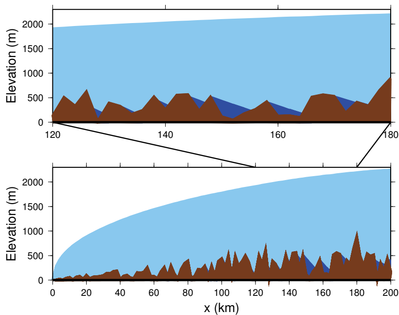
(a) Model results
