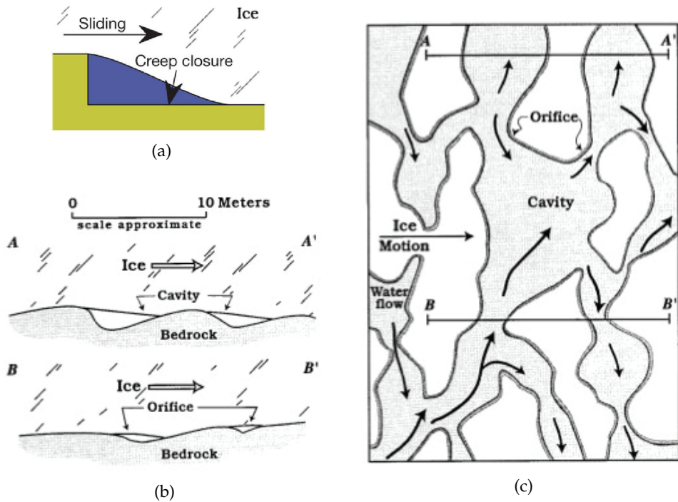
Figure 13: Distributed water flow through linked cavities: (a) Schematic basal ice cavity behind a bedrock protrusion. Its size is defined by the interplay between ice sliding and creep closure (Fig. after Schoof, 2010). (b) and (c) Idealized network of linked cavities at the ice base. The white areas in the plan view show grounded ice, the gray areas are water-filled basal cavities connected by orifices and the arrows indicate the water flow directions. The cross sections reveal the limiting impact of the orifices on the water flow of the system (Figures by Fountain and Walder, 1998).
